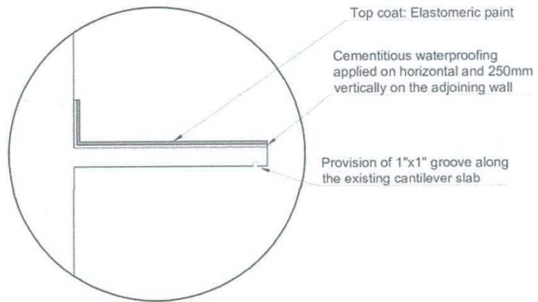
Cantilever Slab Waterproofing Detail
