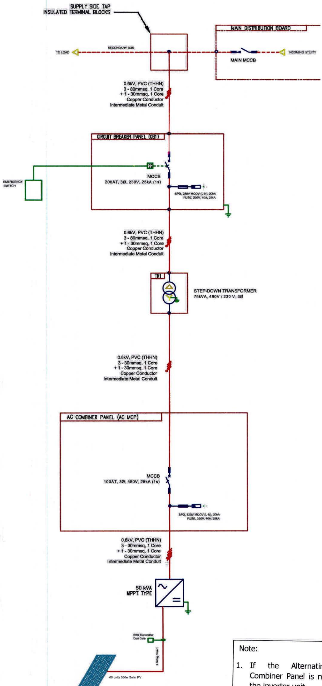
SINGLE LINE DIAGRAM
