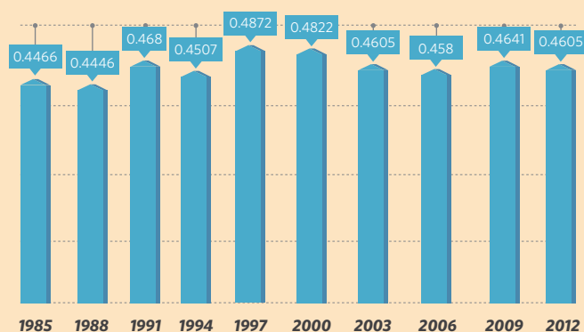
Gini Coefficient
