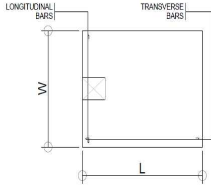
REINFORCEMENT LAYOUT PLAN
