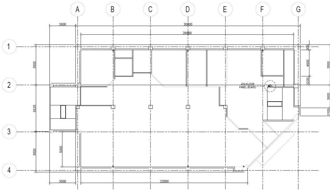
1 FOURTH FLOOR ELECTRICAL PLAN E-6 SCALE 1:100MTS
