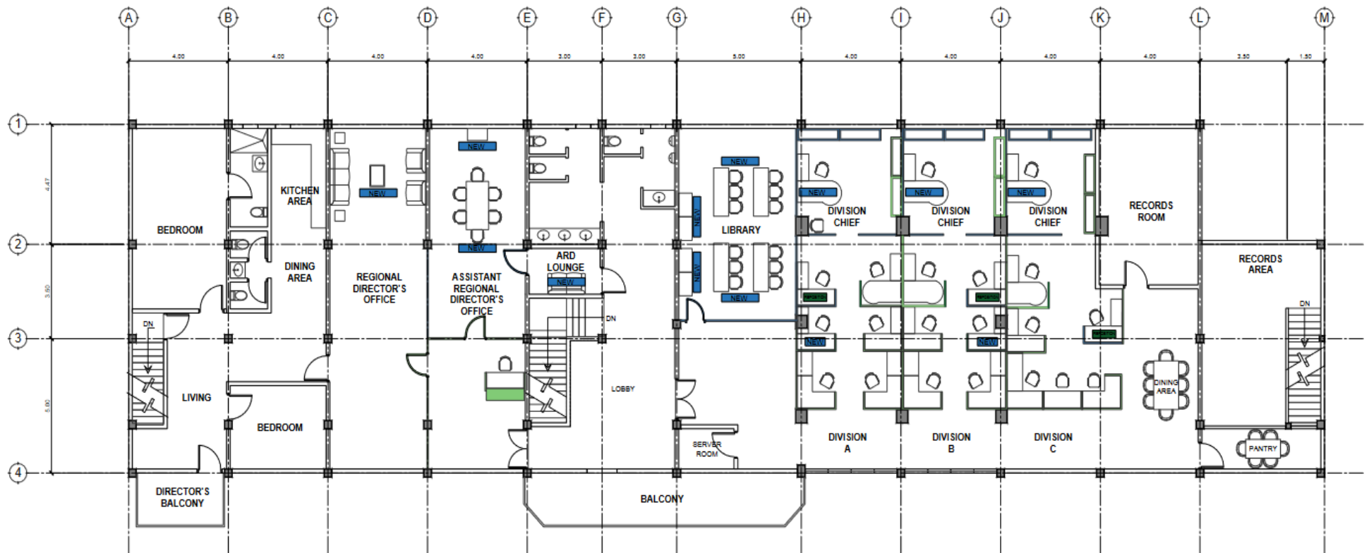
A-1-2 02 14 SCALE 1:150 MTS. SECOND FLOOR FURNITURE LAYOUT
