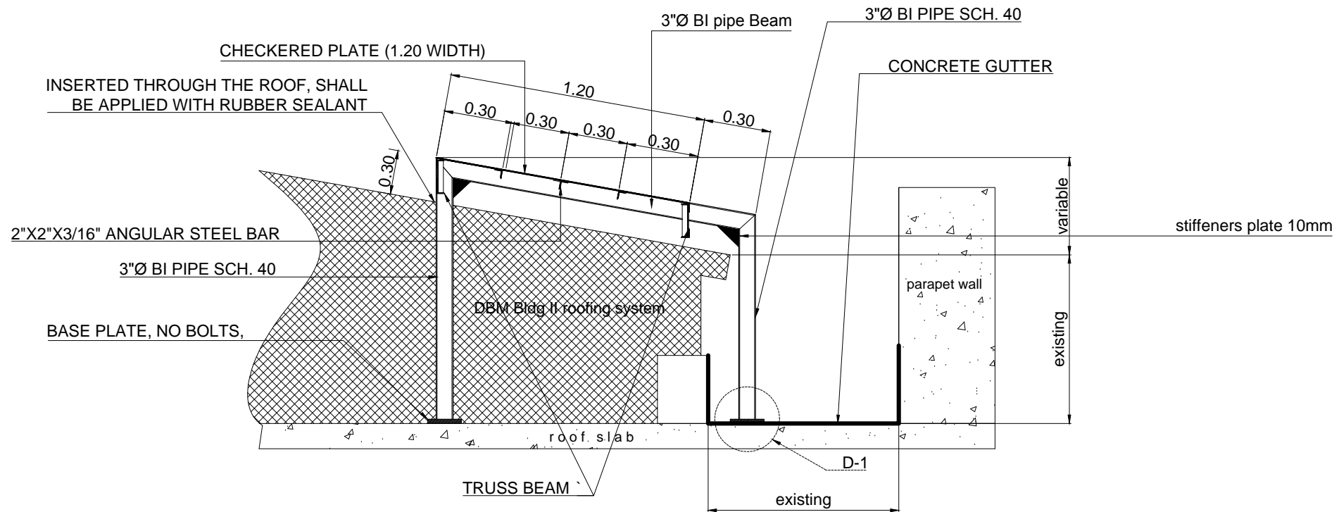
6 ELEVATION PLAN OF CATWALK SCALE: NTS
