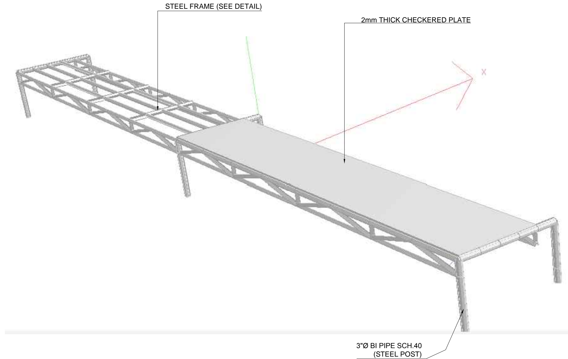
5 S 1 PERSPECTIVE VIEW OF CAT WALK SCALE : NTS
