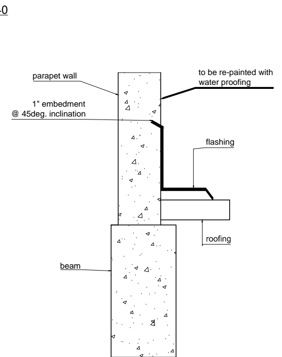
9 END WALL FLASHING DETAIL S 1 SCALE: NTS
