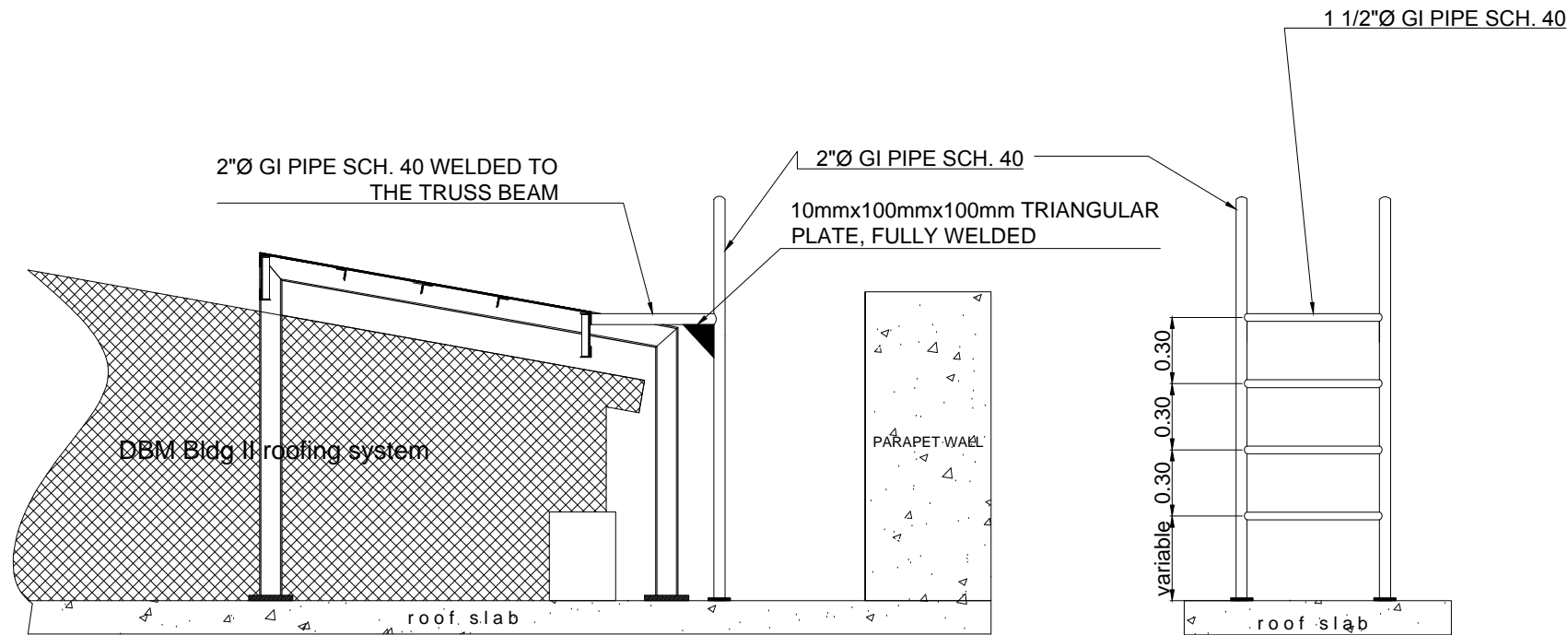
10 STEEL LADDER DETAIL S 1 SCALE: NTS
