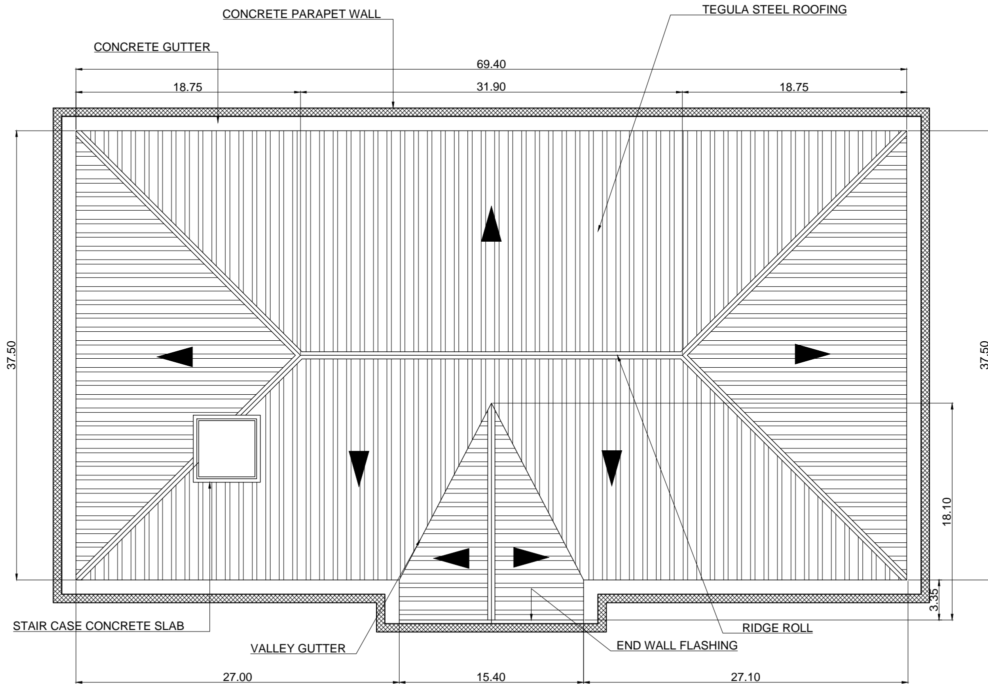
1 S 1 EXISTING DBM ROOF PLAN SCALE : NTS
