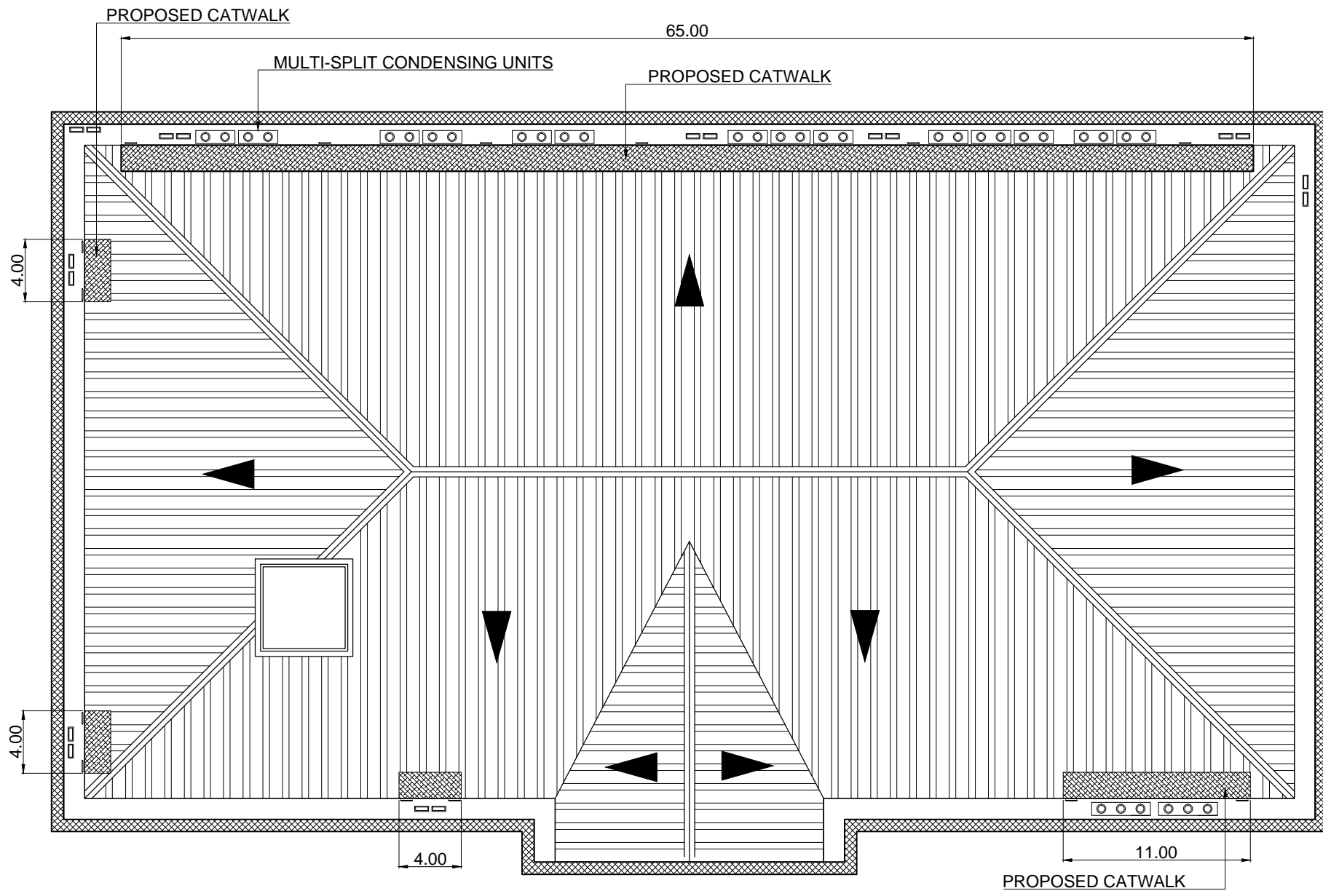
2 S 1 PROPOSED CATWALK LAYOUT SCALE : NTS
