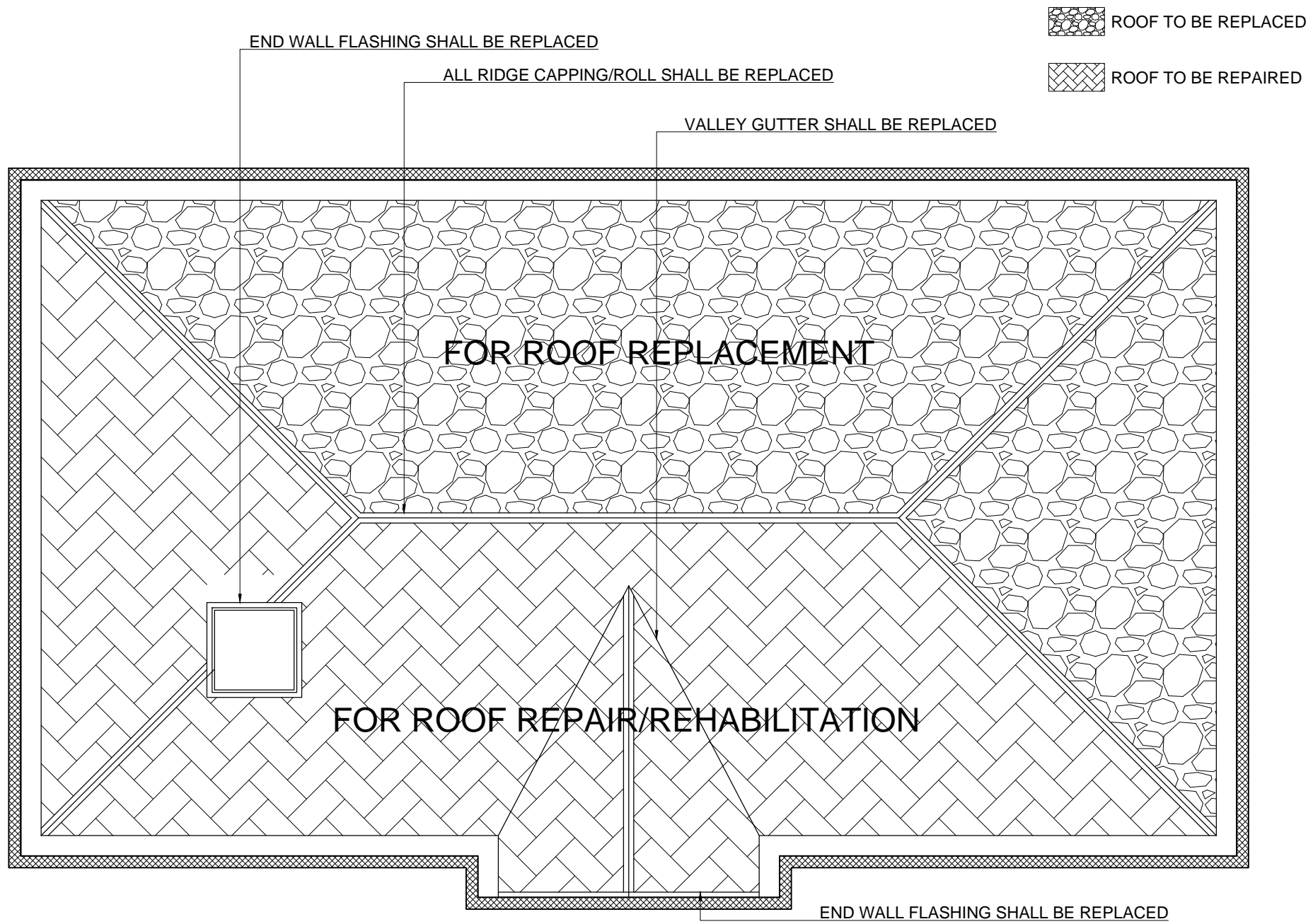
3 S 1 PROPOSED REPAIR/REPLACEMENT OF ROOF SCALE : NTS
